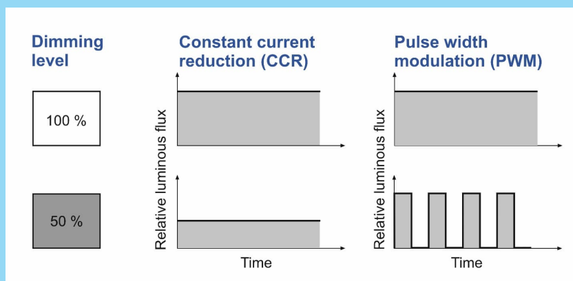
Figure 2 – Two different dimming modes
